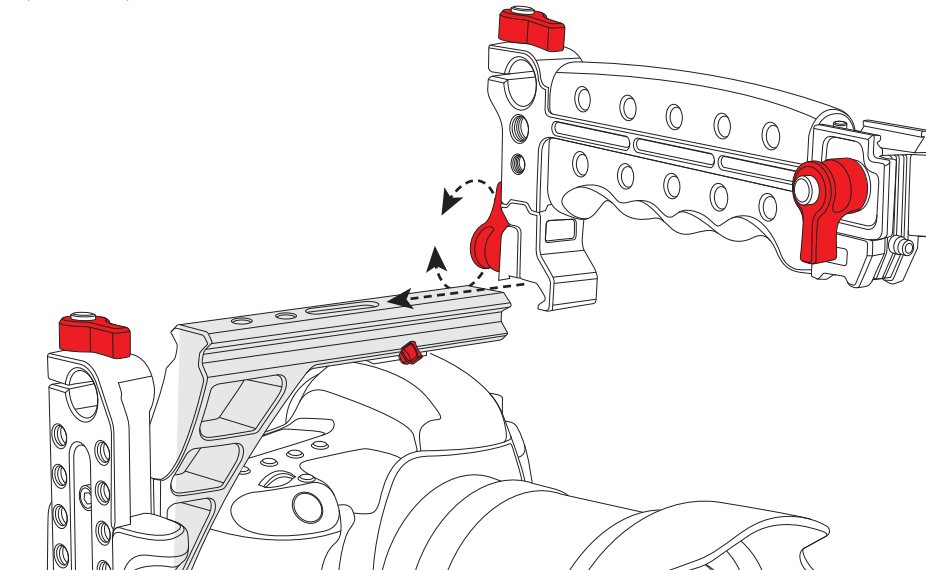
Figure 4:a Mounting your Recoil Handle (Indie Kit)
