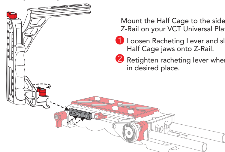
Figure 3:b Mounting Half Cage (Indie Kit)
