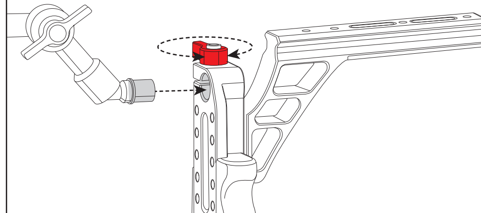
Figure 4:a Mounting your Recoil Handle (Indie Kit)
