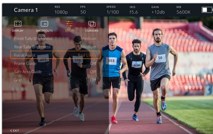
Submenu “Setup”.
