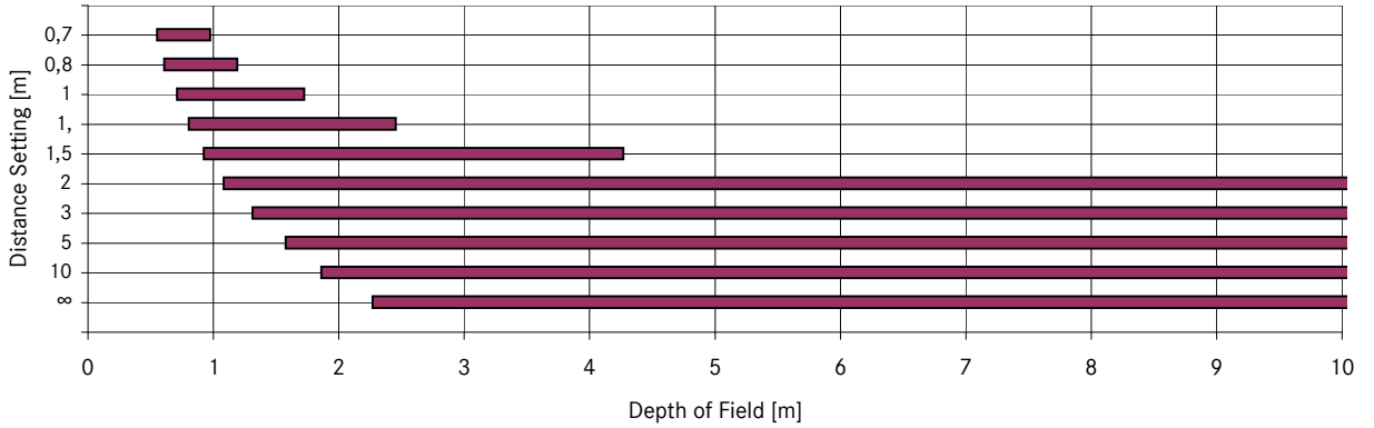
Aperture Stop 11
