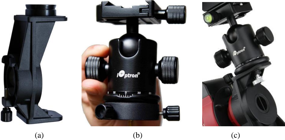
Figure 16. Various mounting methods
