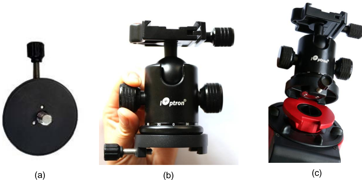
Figure 12. Attach a ball head to the mounting block
