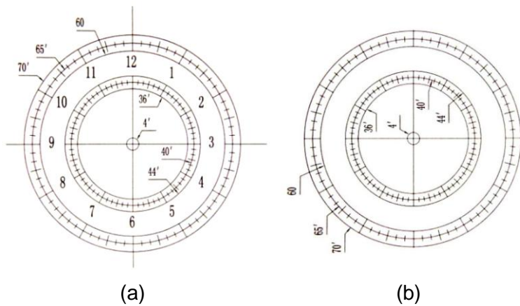
Figure 19. Polar scope dial
