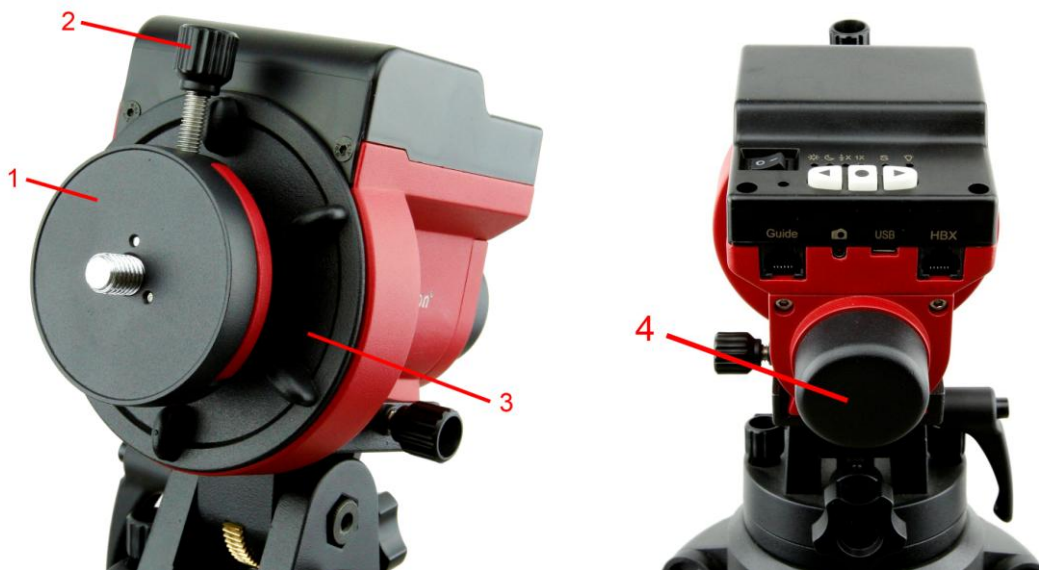
Figure 4. Front and back view of a SkyGuider™ Pro mount head
