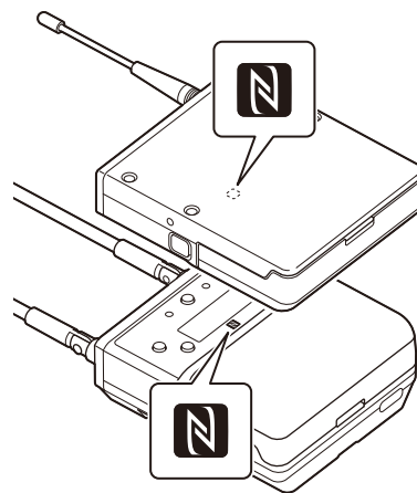
Example using a body-pack transmitter (UTX-B40). Similarly, place the N-Marks in close proximity when using other types of transmitters.
