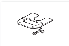
Reinforcement Plate for the CDX-36150 Recorder 3 including 0.64 cm, 1/4" fixation screws (x 2)
