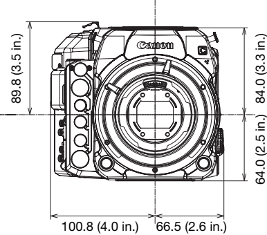
Front view C700 PL C700 GS PL C700 FF PL
