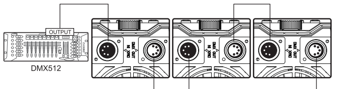
Daisy chaining multiple lights using DMX
