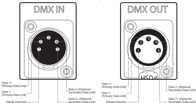
Daisy chaining multiple lights using DMX
