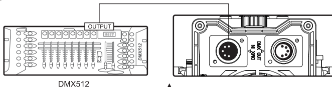
Connecting DMX to only one 600d Pro
